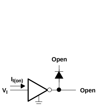
Figure 3. I_I Test Circuit
